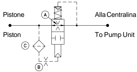
Schema Idraulico - Schematic Diagram
