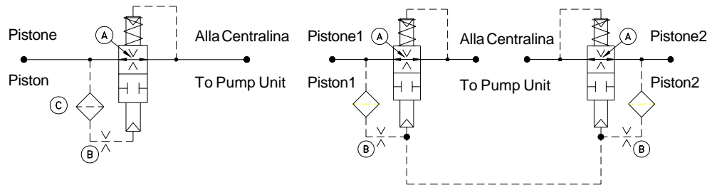
Schema Idraulico 1 e 2 Pistoni Schematic Diagram 1 and 2 Pistons
