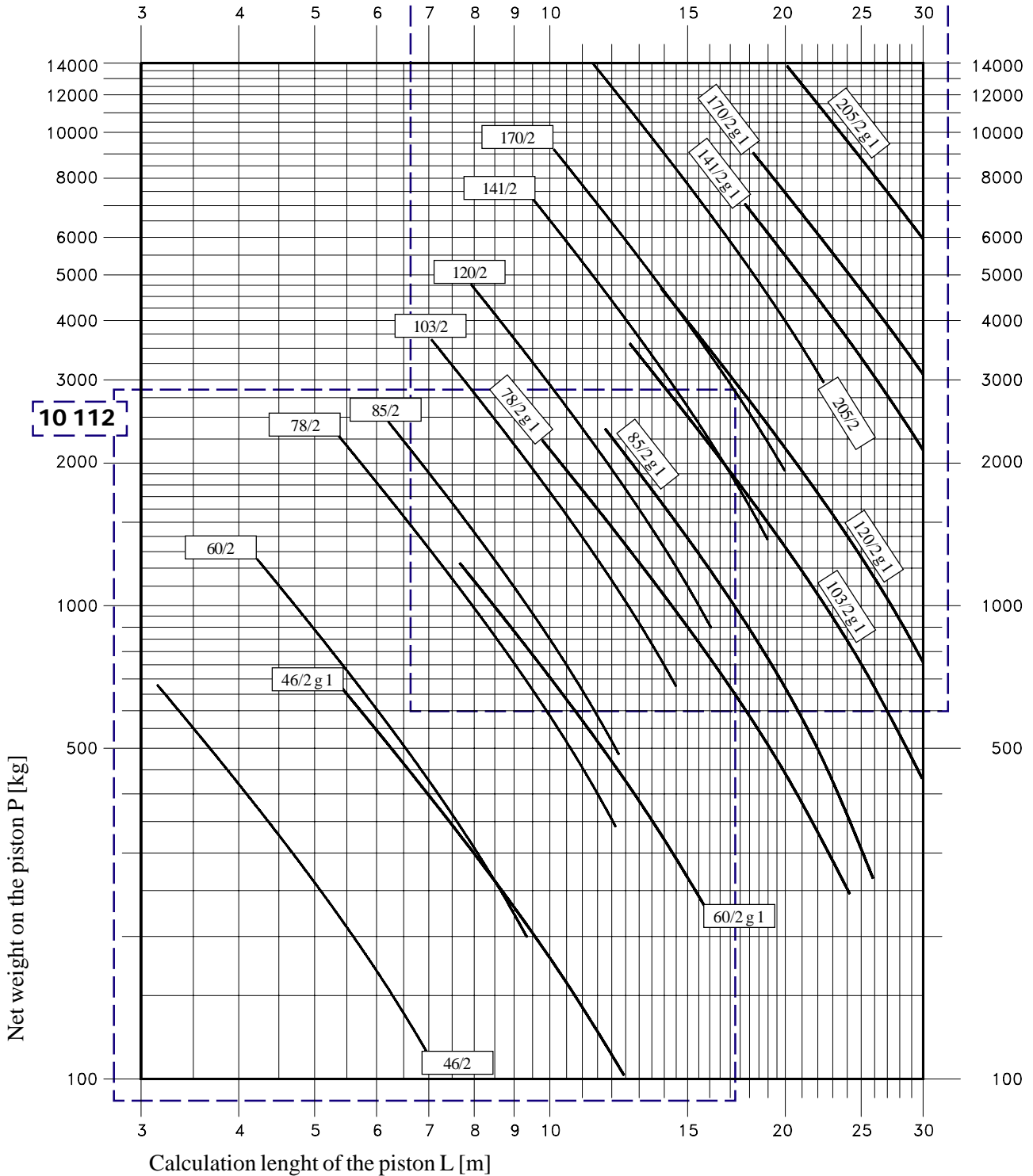
Piston without guide es. 46/2
