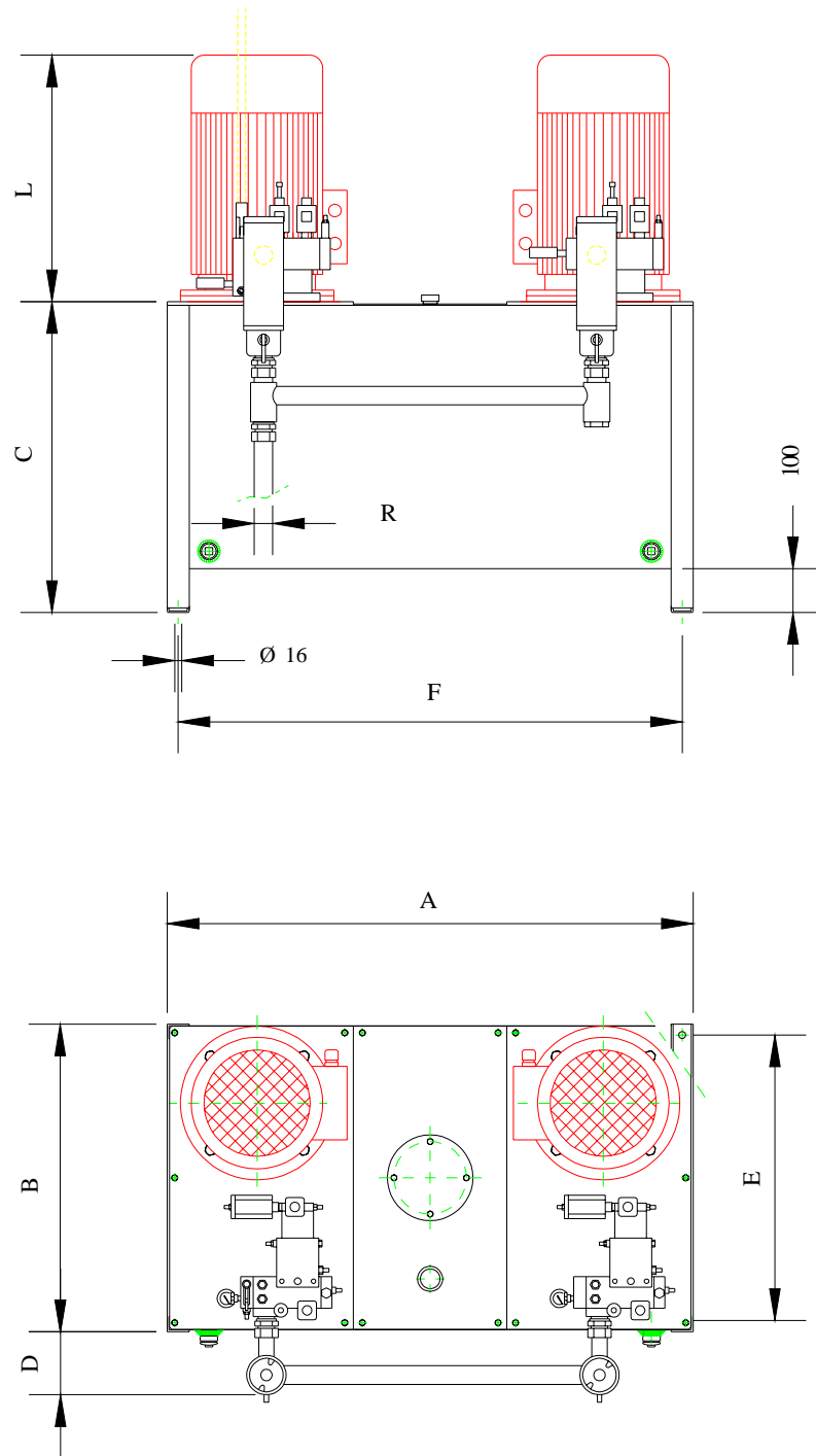
DOUBLE MOTOR-PUMP GROUP (2MP)
