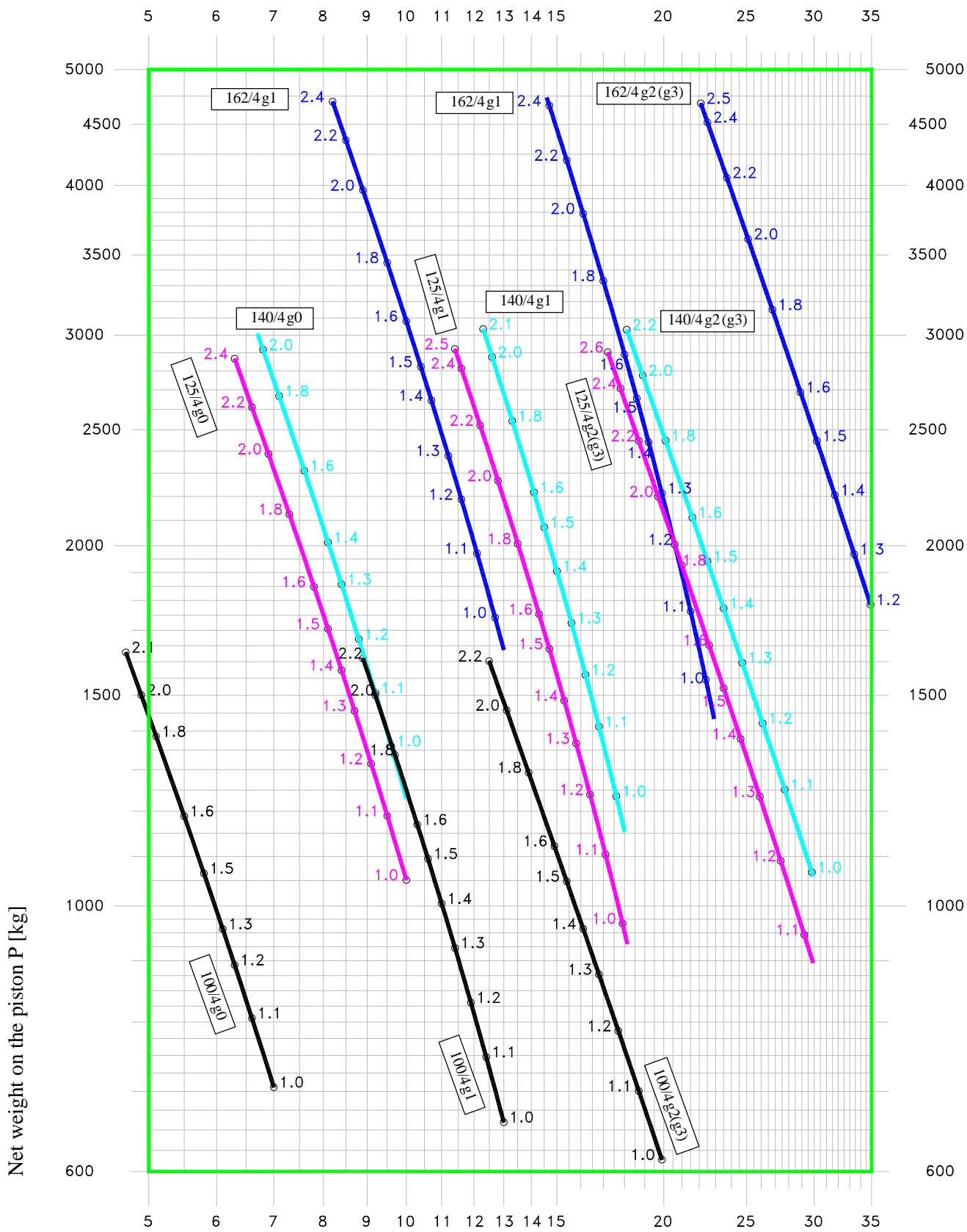
Calculation length of the piston L [m] (For 28 m higher travels to consult Our technical Office)
